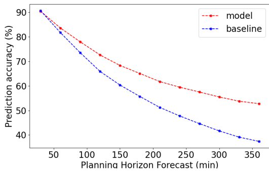
(c) JFK Model accuracy Vs Baseline
