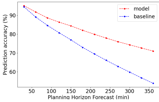
(a) CLT Model accuracy Vs Baseline
