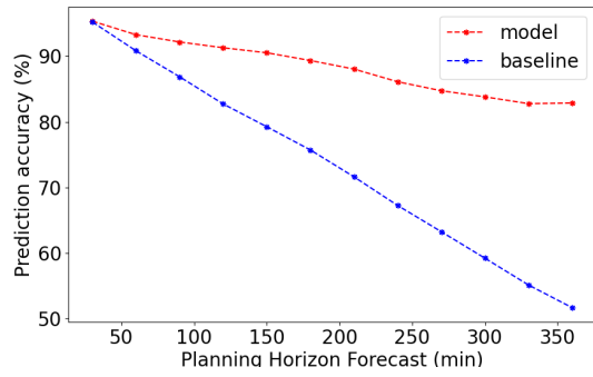
(b) DFW Model accuracy Vs Baseline
