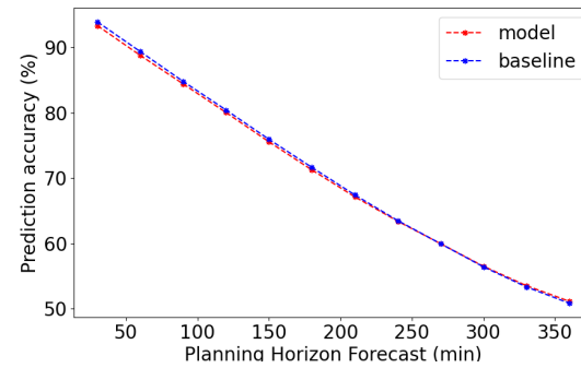
(e) DAL Model accuracy Vs Baseline
